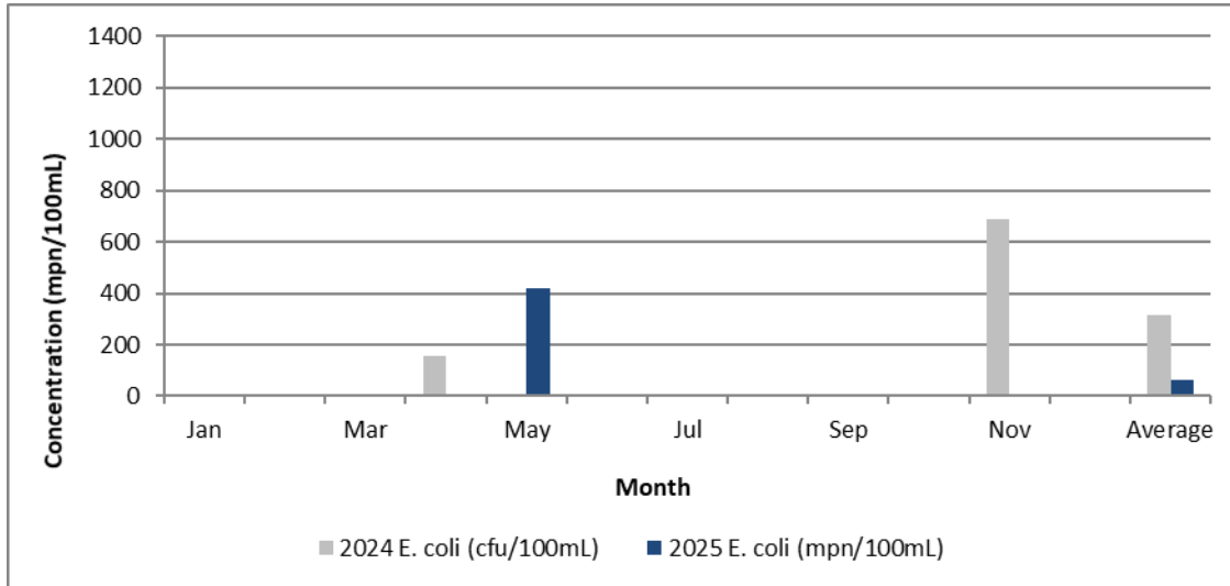
Figure 15: Effluent E. coli Concentrations 2024 to 2025
