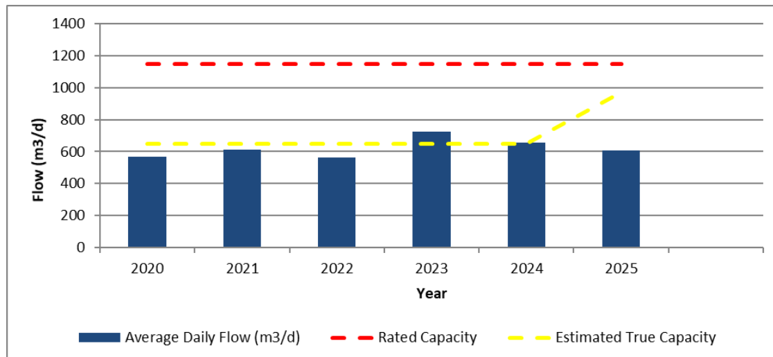
Figure 1: Influent Flows 2020-2025
