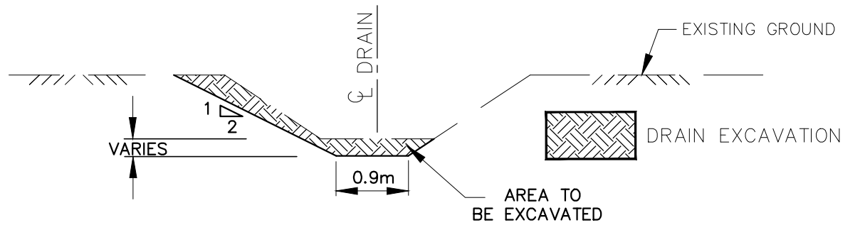
TYPICAL DRAIN CROSS SECTION STATION 0+054 TO 0+237 NTS
