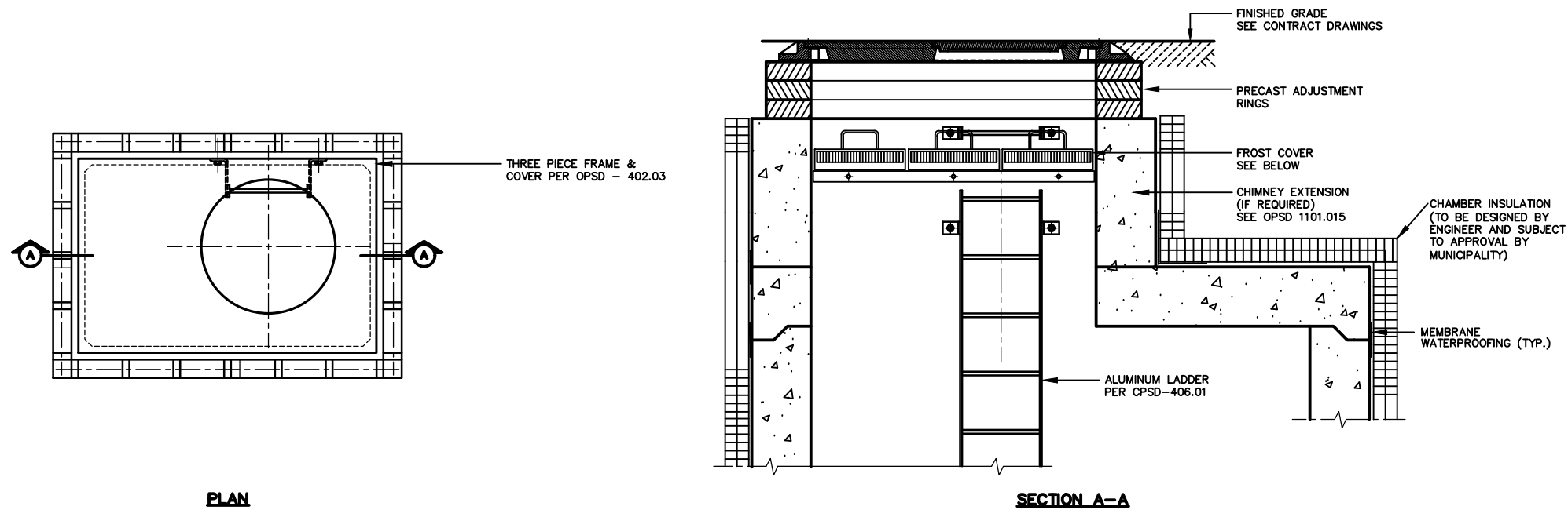
CHAMBER COVER DETAIL SCALE: NTS
