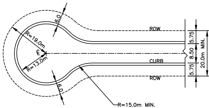
TYPE 'A' MINIMUM (SEE NOTE 2)
