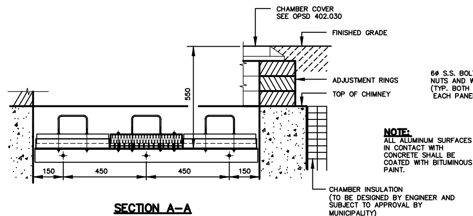
FROST COVER DETAIL SCALE: NTS
